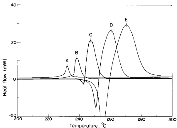
Fig. 1. Influence of the heating rate on the endotherm and the exotherm observed in the thermal decomposition of nitroguanidine. Aluminum crimped pan, nitrogen atmosphere, sample size 1.5 mg. Heating rate: A, 2.5 °C min -1 ; B, 5 °C min -1 ; C, 10 °C min -1 ; D, 20 °C min -1 ; E, 40 °C min -1 .
